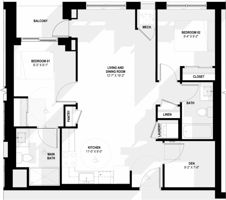
UNIT TYPE G (BARRIER-FREE) SCALE: 1/32" = 1'-0"
