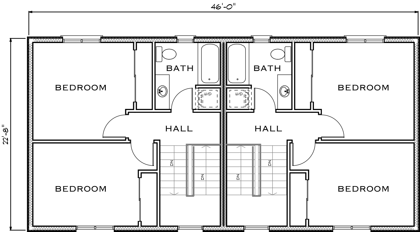
UPPER FLOOR PLAN
